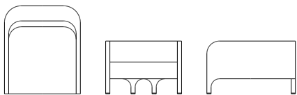
CURVA 80x105xh38/63cm
